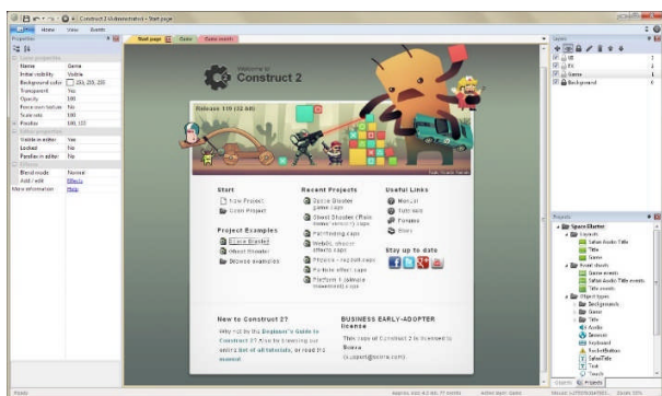
Figura 1: Framework Construct 2.
